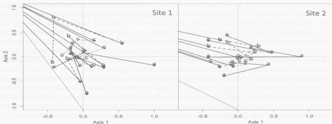
Figure 1. Principal component analysis (PCA) of Sites 1 (on the left) and Site 2 (on the right) along the first two axes. Full dots are plots surveyed in 2013; empty dots are plots surveyed in 2014 and 2015. Letters a (mowed and hay added, solid line), b (mowed, dashed line) and c (control, dotted line) indicate cultural practices. Dots of each block are joined with a line along time gradient.
